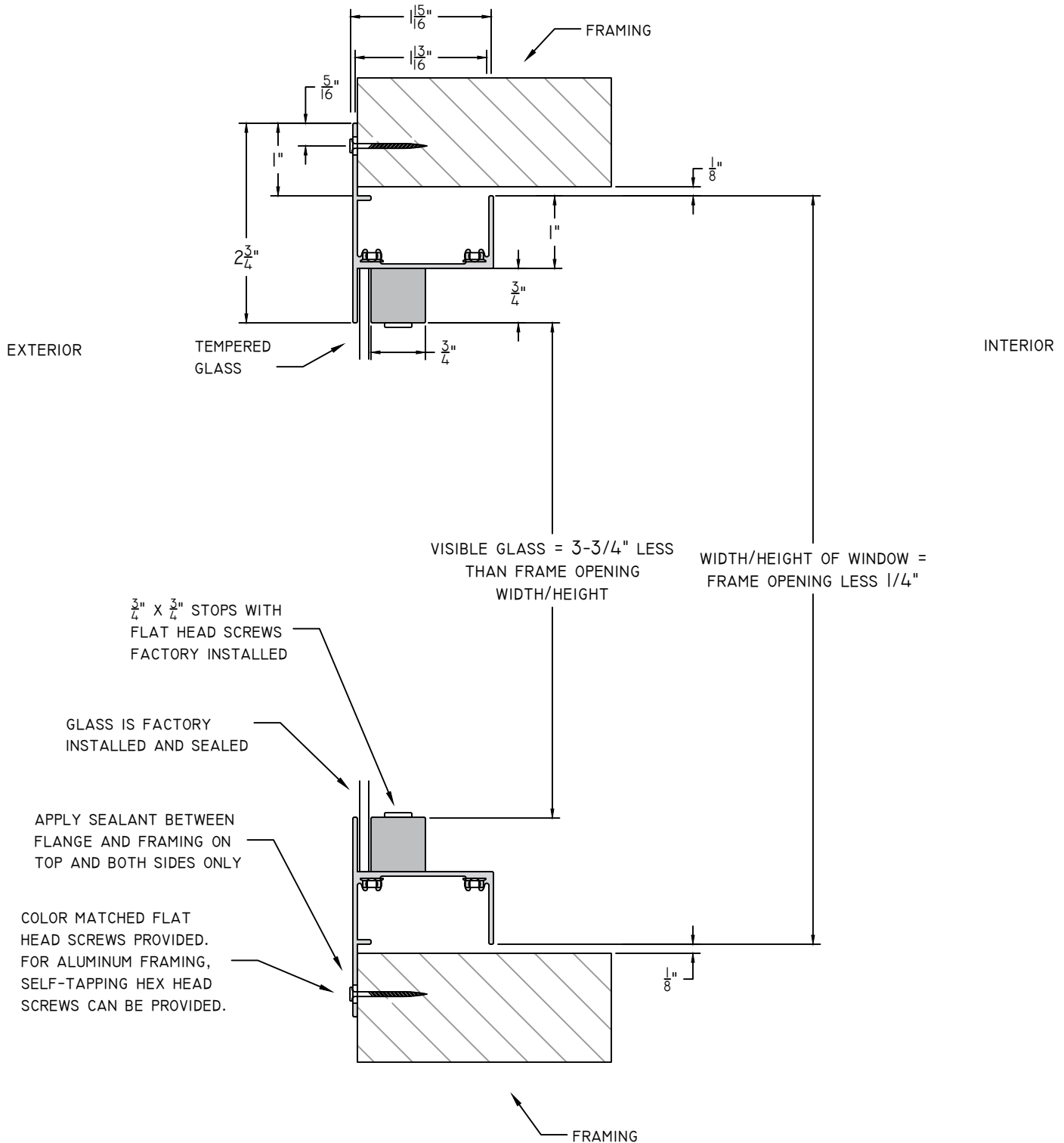
FRAME CROSS SECTION
